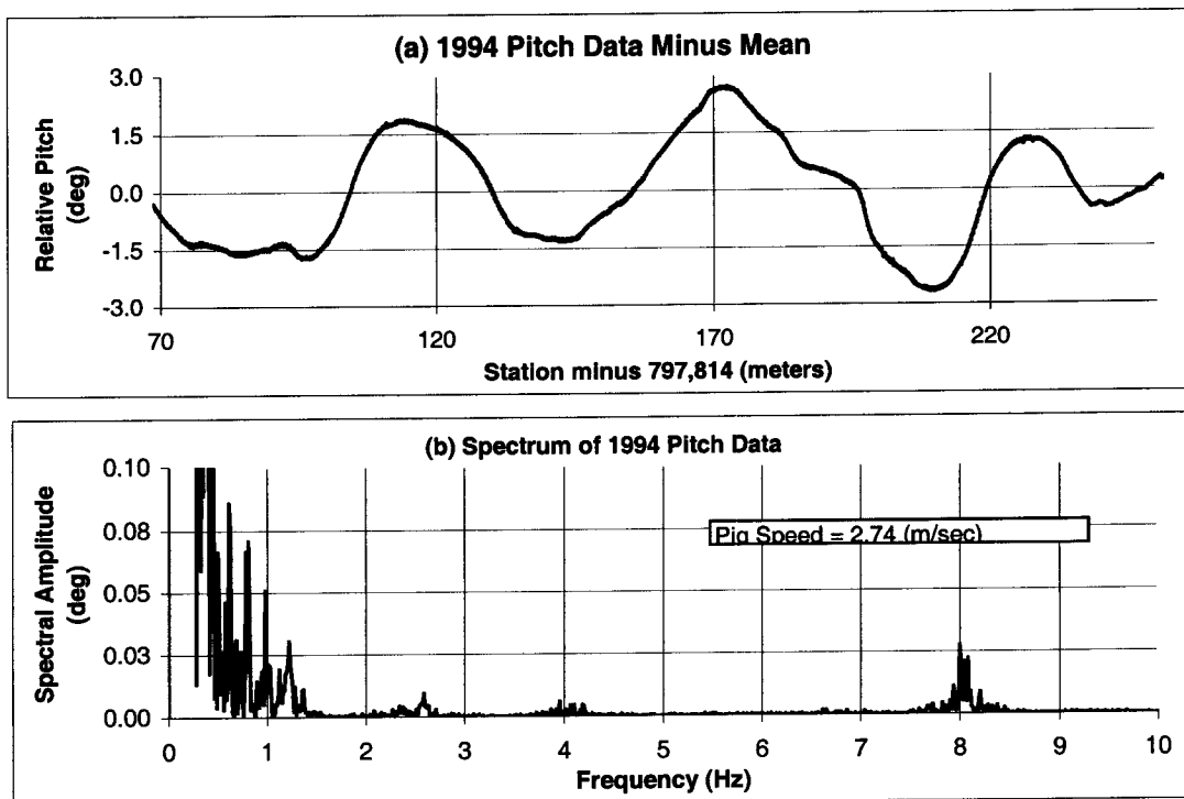
Figure 2: Illustration of Pitch Data from Salcha River Crossing
