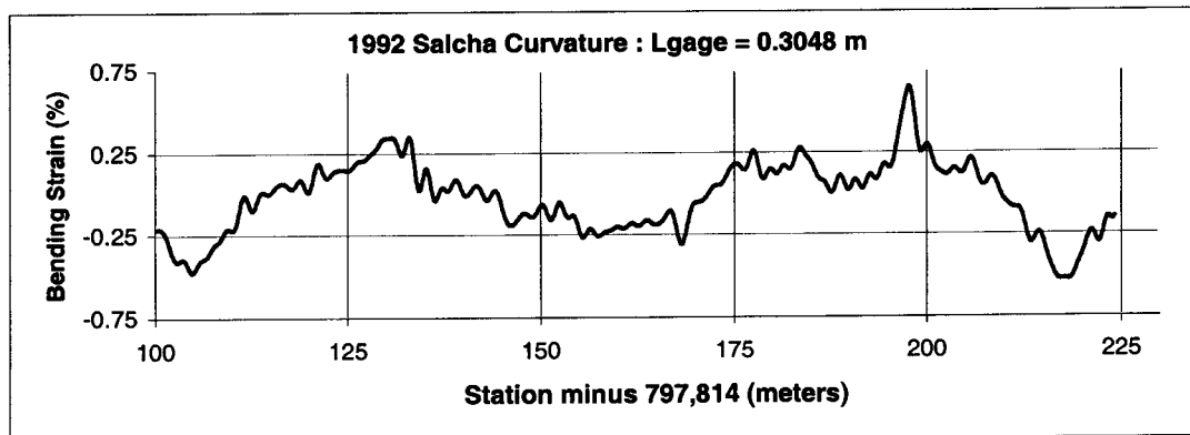
Figure 4: Illustration of Filtered Curvature Data from Salcha River Crossing
