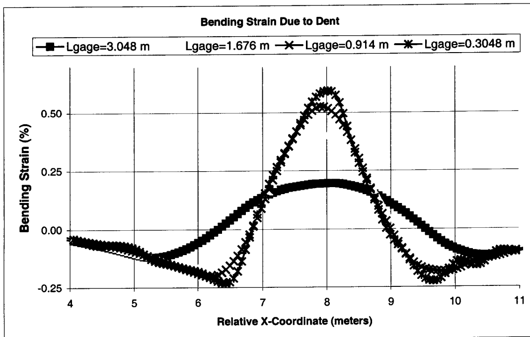
Figure 6: Illustration of Profile Due to Dent at Salcha River High Curvature Zone
