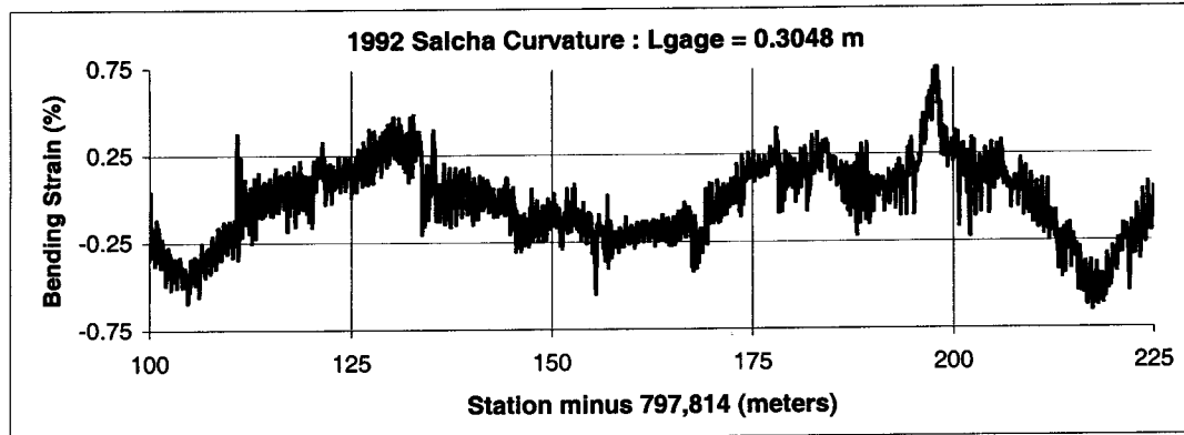
Figure 3: Illustration of Unfiltered Curvature Data from Salcha River Crossing
